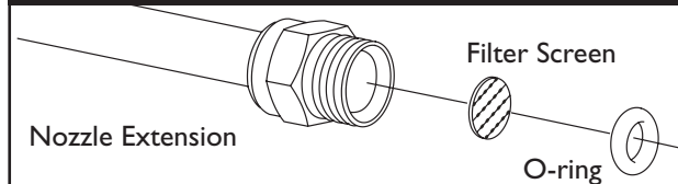
Figure 19 — Clean In-Line Filter
